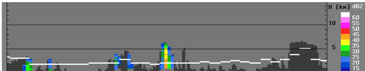
Figure 5. Vertical cross section along the line AB in Fig. 2, where the left end is point A and the right end correspond to point B in Fig. 2. The gray area is the clouds, as measured by their top temperature. The colors represent the precipitation reflectivity, in dBZ, as measured by the TRMM radar. The white line is the brightness temperature of the TRMM Microwave Imager 85 GHz vertical polarization, plotted at the altitude of that
