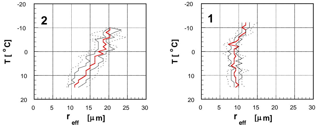
Figure 6. Analysis of the temperature ( T ) - droplet effective radius ( r_e ) relationship, for the clouds in the two boxes plotted in Fig. 4, respectively. Area 1 is smokey (on the right of Figure 4, whereas Area 2 is smoke-free. Plotted are the 10% 25% 50% 75% and 90% percentiles of the r_e for each 1^\circ\text{C} interval. The median is indicated by the thick red line. From Rosenfeld (1999).
