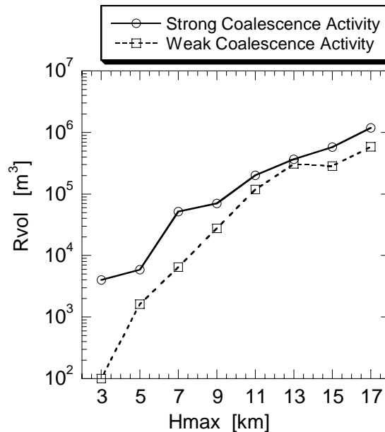
Fig. 7. The mean rain volumes of convective cells as a function of maximum precipitation echo top height for cells growing on days with weak coalescence activity and on days with strong coalescence activity. The data are plotted at the center point of 2 km intervals of maximum echo top height. For the purpose of showing the trend on a logarithmic scale, a value of 10^2 \text{ m}^3 was used instead of the zero value of RVOL for the 3 km maximum echo top height interval for cells growing on days with weak coalescence activity. From Rosenfeld and Woodley (2003).
