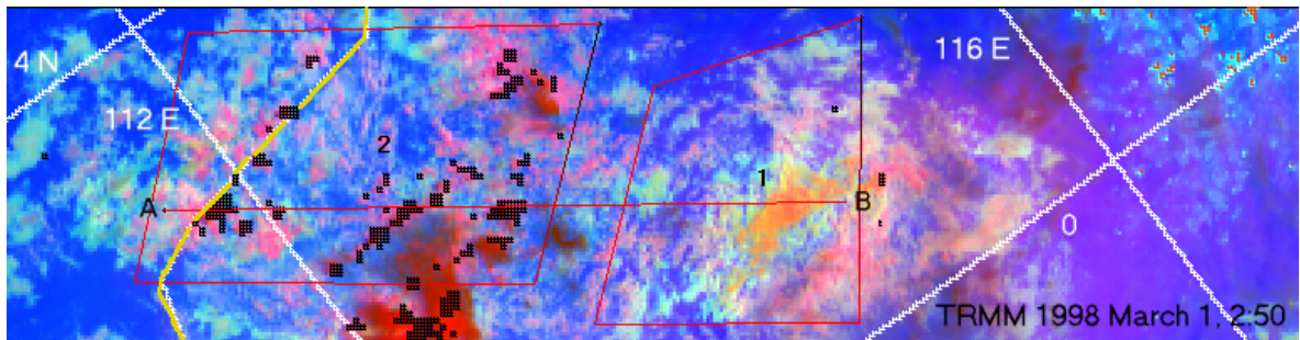
Figure 4. The TRMM VIRS image of fires, smoke and clouds over Kalimantan, Indonesia, from 1 March 1998, 02:50 UT. The color is composed of: red for visible reflectance, green for 3.7\ \mu\text{m} reflectance (approximating the cloud drop effective radius, r_e ), and blue for the inverse of 10.8\ \mu\text{m} brightness temperature. The northwest coast of the island is denoted by the yellow line. The small orange areas on the upper right (east) corner are hot spots indicating the fires. The smoke, streaming from the hot spots south-westward, is indicated by the fuzzy purple color of the background. The smoke-free background is blue. This color scheme (see full detail in Rosenfeld and Lensky, 1998) shows clouds with small droplets ( r_e < 10\ \mu\text{m} ) as white, becoming yellow at the supercooled temperatures. Clouds with larger droplets ( r_e > 15\ \mu\text{m} ) are colored pink, and cold ice clouds appear red. The black hatching marks the areas in which the TRMM radar detected precipitation. From Rosenfeld (1999).
