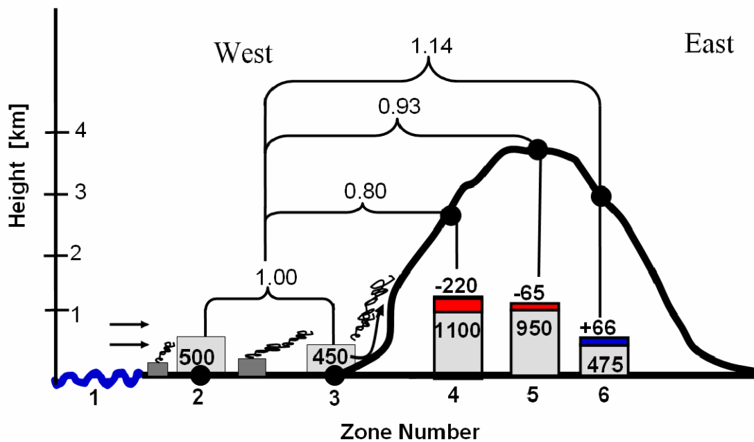
Figure 9. The effects of pollution on rainfall in the Sierra Nevada Mountains in California. The figure is a schematic topographic cross section showing the effects of urban air pollution on precipitation as the clouds move from west to east from the coast to the Sierra Nevada and to the eastern slopes. The boxes show the amount of the annual precipitation ( \text{mm yr}^{-1} ) in each topographic location, and the numbers above them show the loss or gain of precipitation ( \text{mm yr}^{-1} ) at each site. Maritime air (zone 1) is polluted over coastal urban areas (zones 2, 3), with no decrease in precipitation. The polluted air rises over mountains downwind and forms new polluted clouds (zone 4), with decreases of \sim 15\% – 20\% (losses of 220 \text{ mm yr}^{-1} ) in the ratio between the western slopes and the coastal and plain areas (appears as 0.80 above the line connecting zones 4 and zones 2-3). The clouds reach to the high mountains in zone 5. All of the precipitation is snow,
