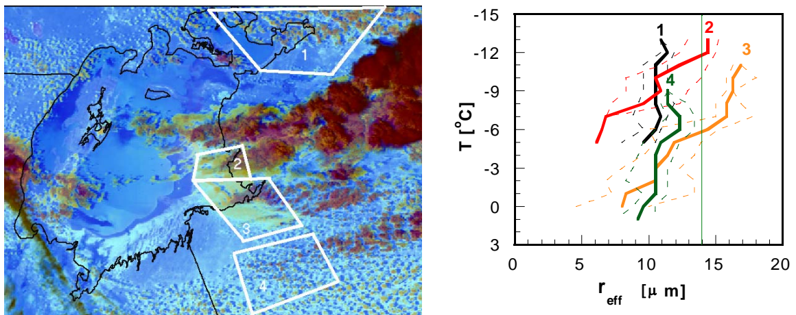
Figure 10. Left: NOAA -AVHRR satellite image (11 May 1998 09:32 UT) showing clouds forming in salt-dust plumes off the eastern shores of the Aral Sea (frames 2 and 3). Clouds outside the dust storm are shown in frames 1 and 4. Right: T - r_e relationship for the clouds in the 4 areas shown in the left panel. T is the temperature and r_e is the cloud particle effective radius. The solid lines show the median r_e for a given T , and the broken lines show the 15 th and 85 th percentiles. The vertical green line marks the 14\text{-}\mu\text{m} precipitation threshold. Curves 2 and 3 for clouds forming in heavy salt-dust show smaller near-cloud-base r_e and much larger cloud-top r_e compared to background clouds of comparable depths (curves 1 and 4). This analysis shows the fast growth of cloud droplets with height above cloud base. From Rudich et al., (2002).
